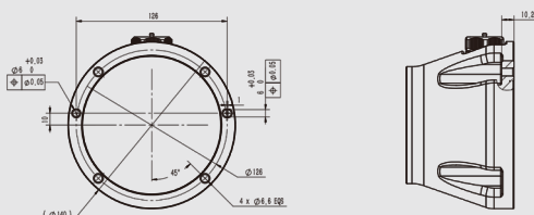
AUBO-i3 Base Top View
