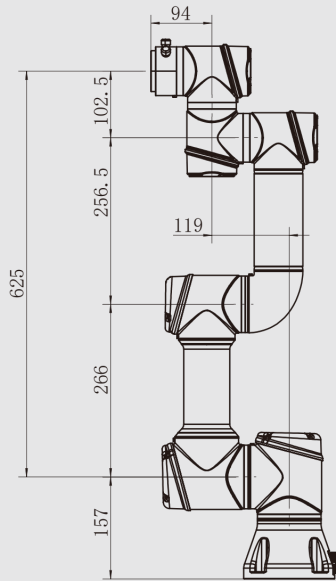
AUBO-i3 Dimensions Diagram
