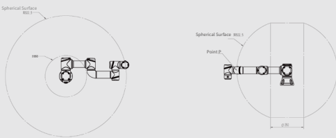
AUBO-i3 Point P Motion Range
