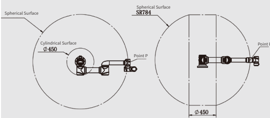
AUBO-i5 Point P Motion Range
