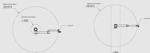
AUBO-iS20L Dimensions Diagram
