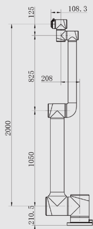
AUBO-iS20L Dimensions Diagram
